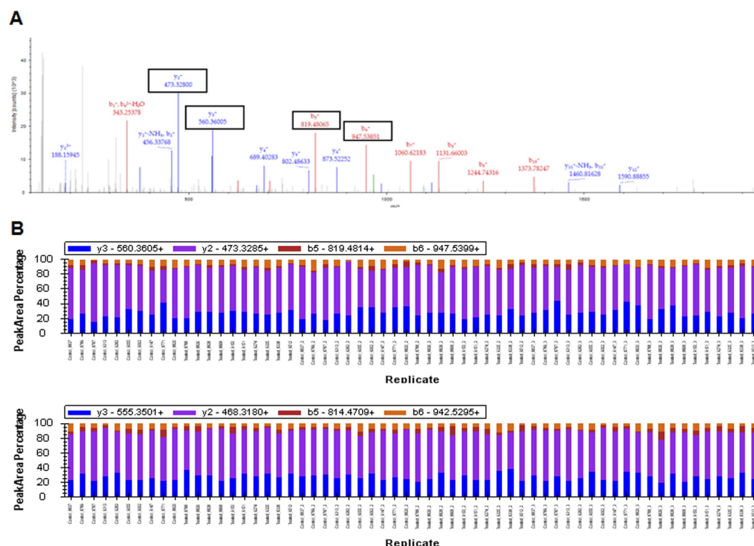
Figure 3. The raw LC-MS/MS spectra of 60S ribosomal protein L18. The peptide “ILTDFDLAESP” from 60S ribosomal protein L18 detected in the discovery analysis via the Orbitrap Velos-Pro is presented along with the same peptides Transition Peak Area Percentage detection from TMT-SRM analysis via the TSQ Vantage.
